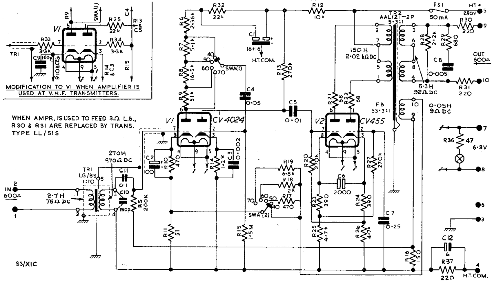
Fig. 23.1 Amplifier AMC/5: Circuit
